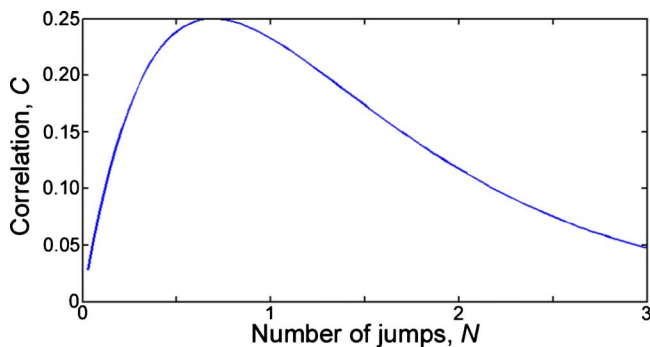
FIG. 4. (Color online) Variation in the correlation, C , as a function of the average number of spectral jumps, N .
